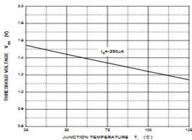
Threshold Voltage
